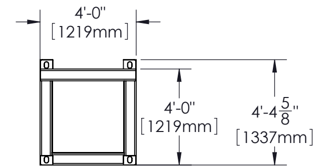
END ELEVATION VIEW
